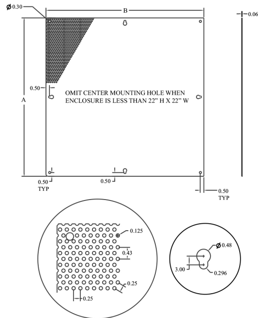
NEMA 1 PERFORATED SUBPANEL
