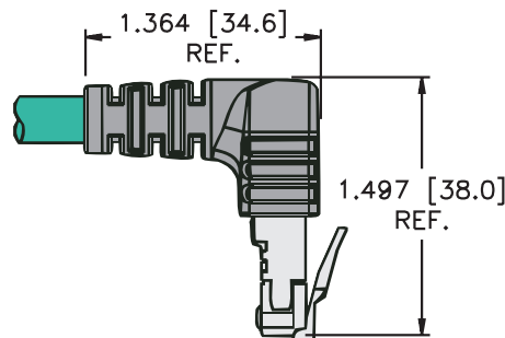
RJ45 connector
