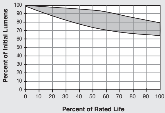
Typical Lumen Depreciation
