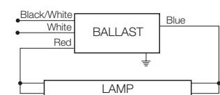
QUICKTRONIC 1x32
