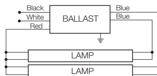
QUICKTRONIC 2x32
