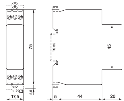
fig. 2. Dimensions (mm)
