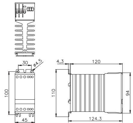
fig. 2. Dimensions (mm)
