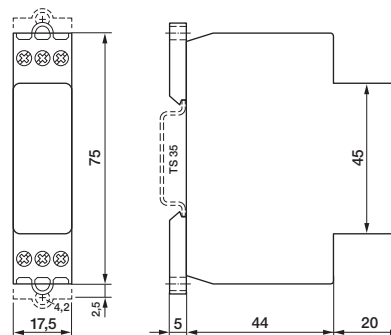
fig. 2. Dimension (mm)
