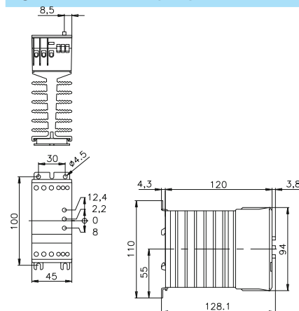
fig. 2. Dimensions (mm)
