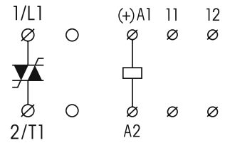
11-12: Thermostat
