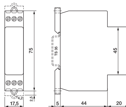
Fig.2 Dimensions (mm)
