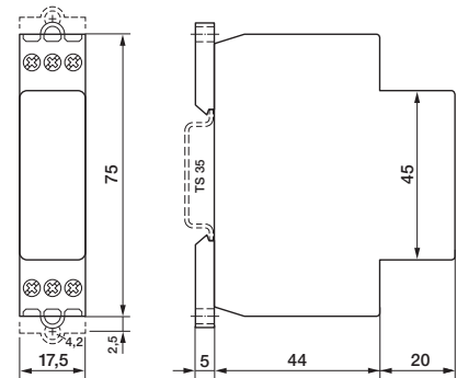
fig. 2. Dimensions (mm)
