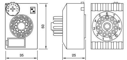
fig. 2. Dimensions (mm)
