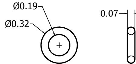
RUBBER O-RING
