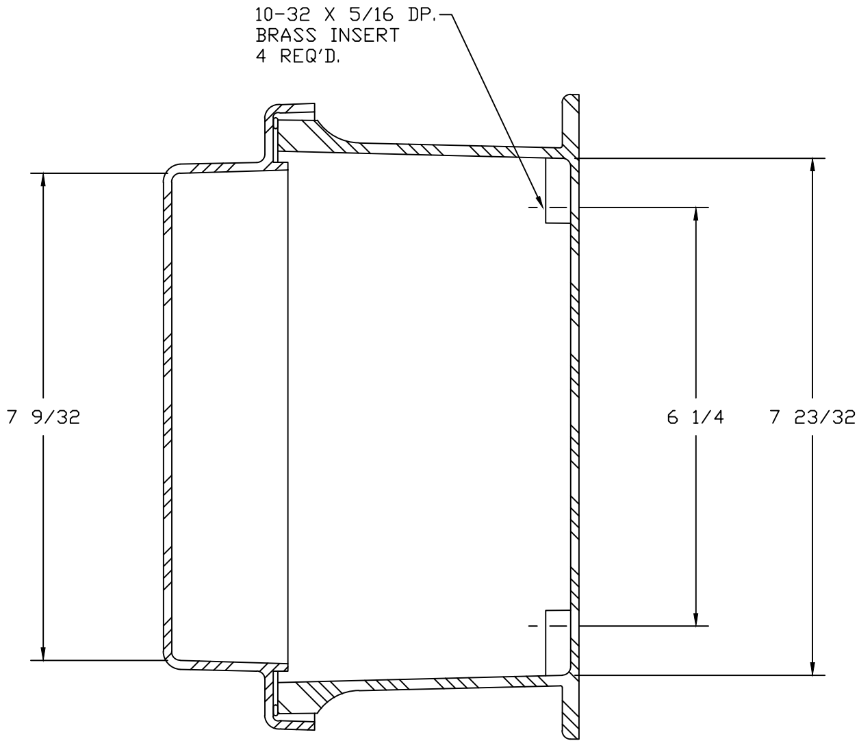
SECTION B-B
