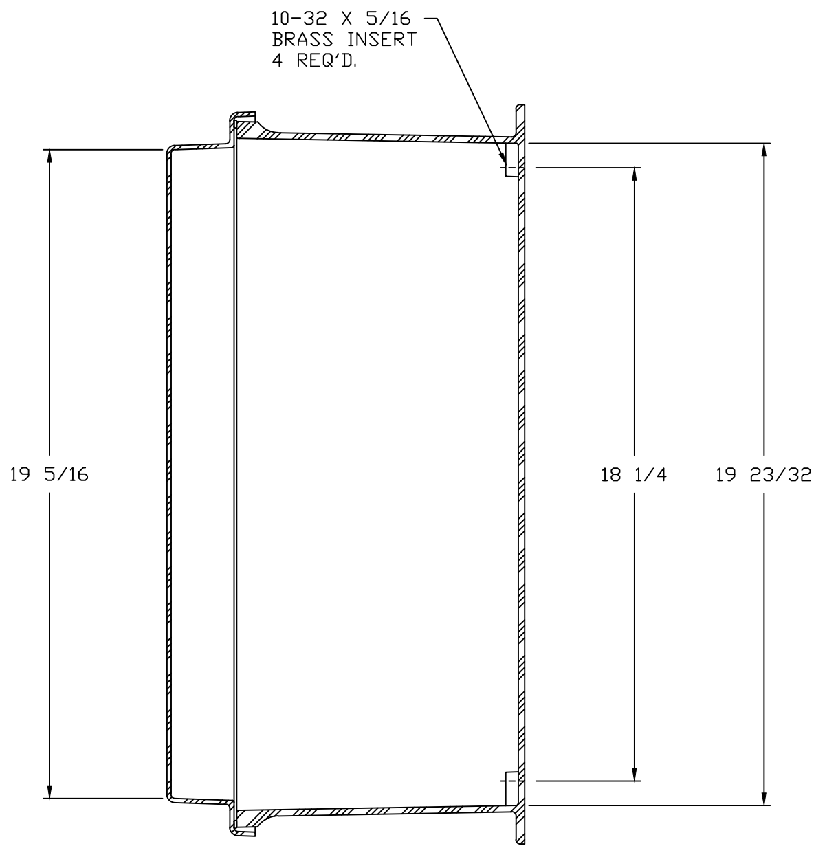
SECTION B-B
