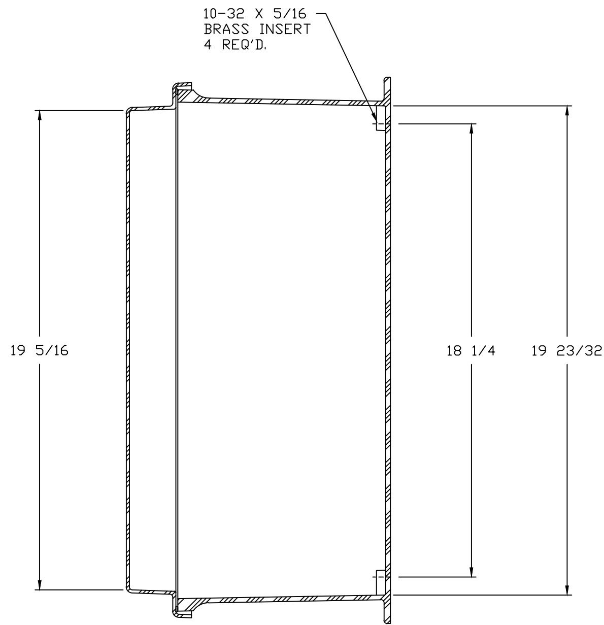
SECTION B-B
