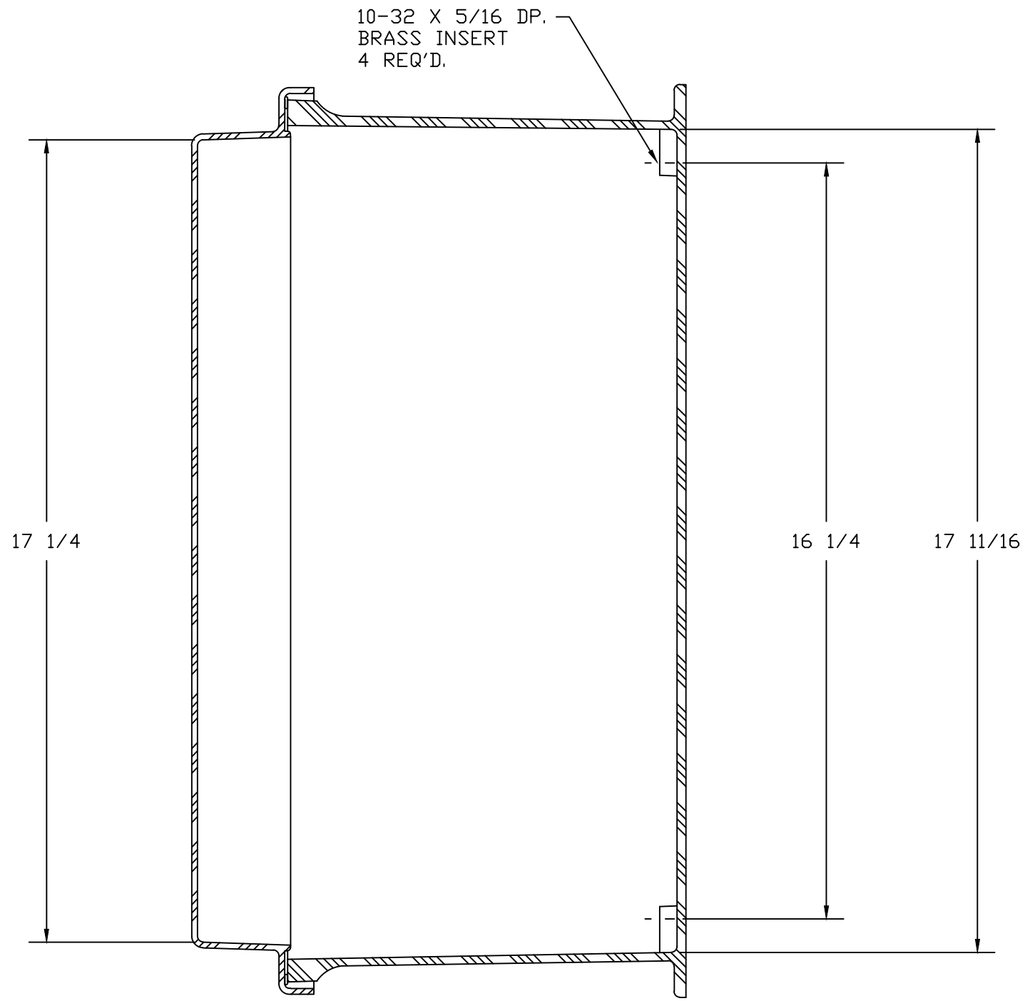
SECTION B-B
