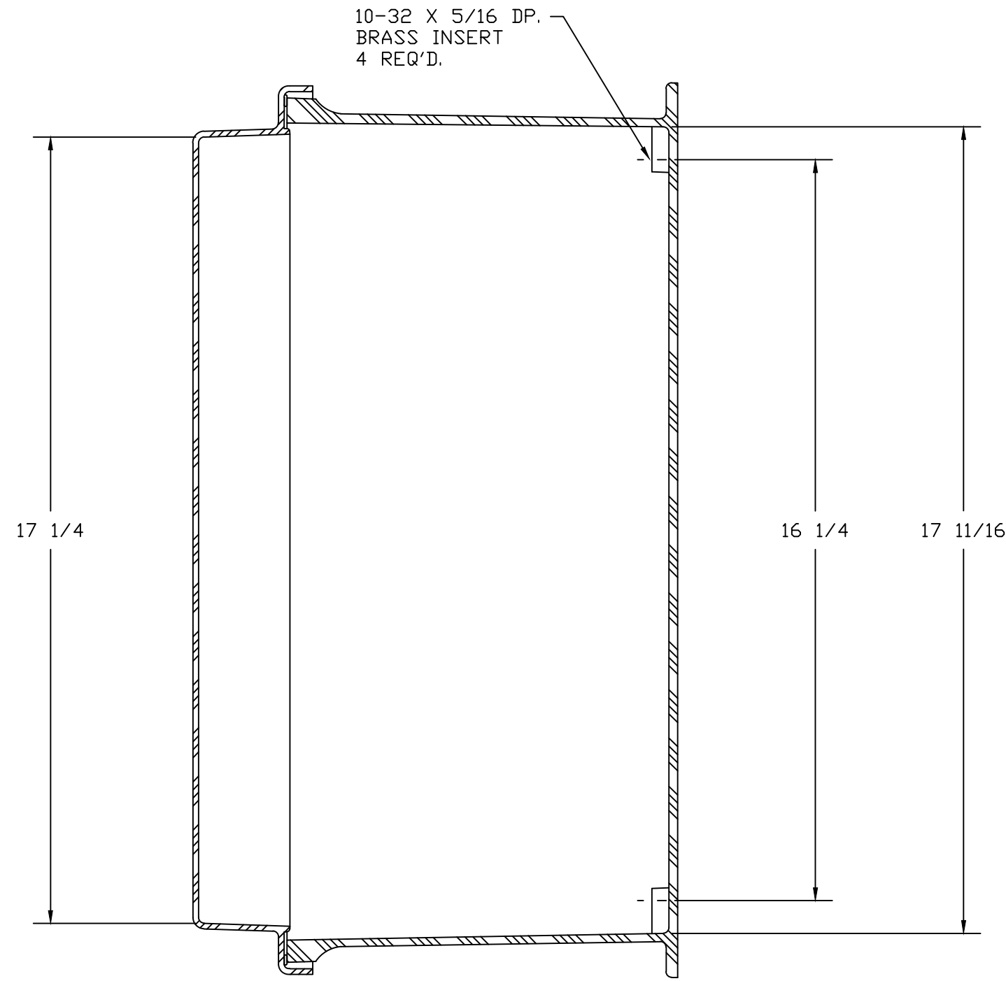
SECTION B-B
