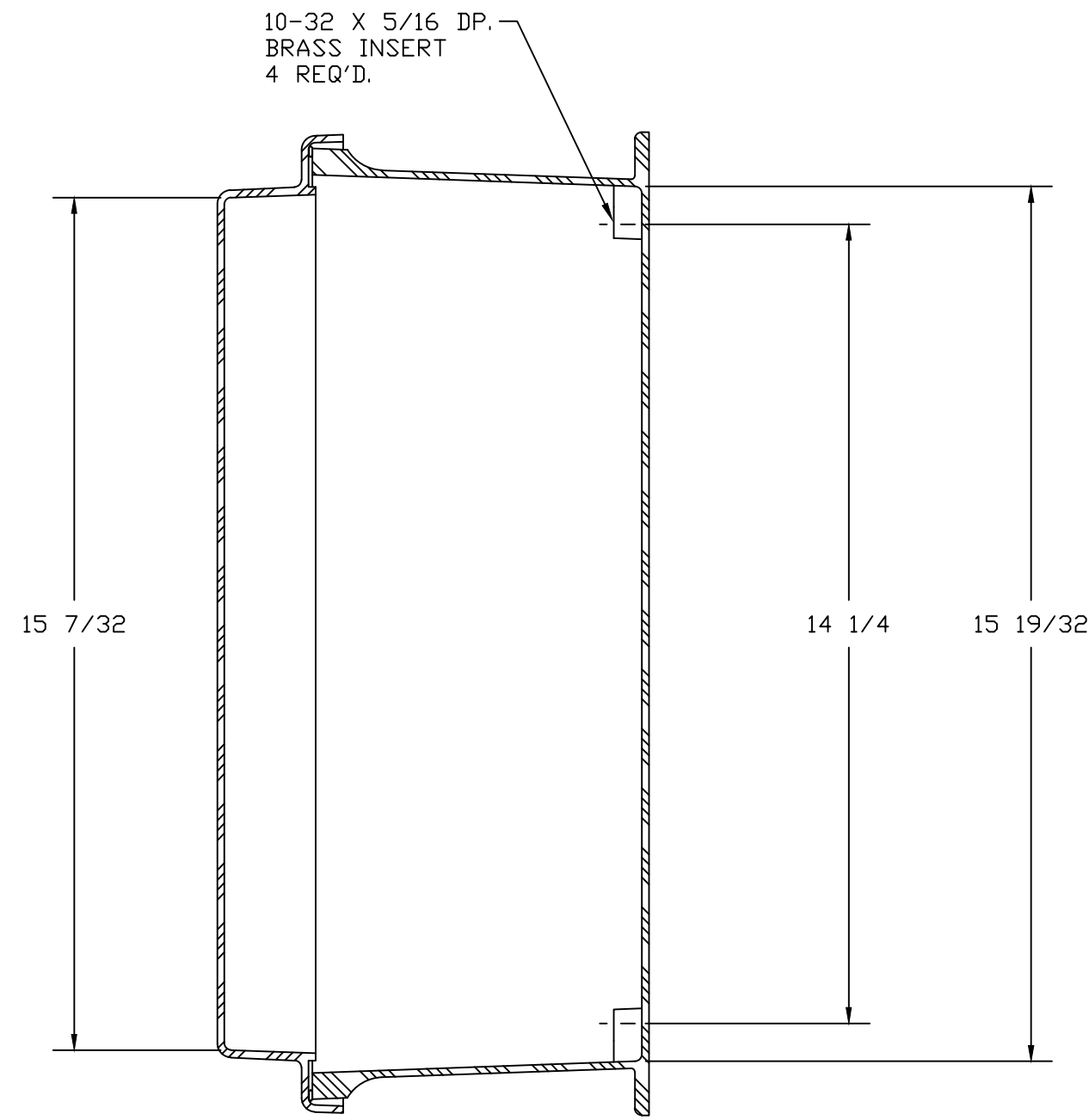
SECTION B-B
