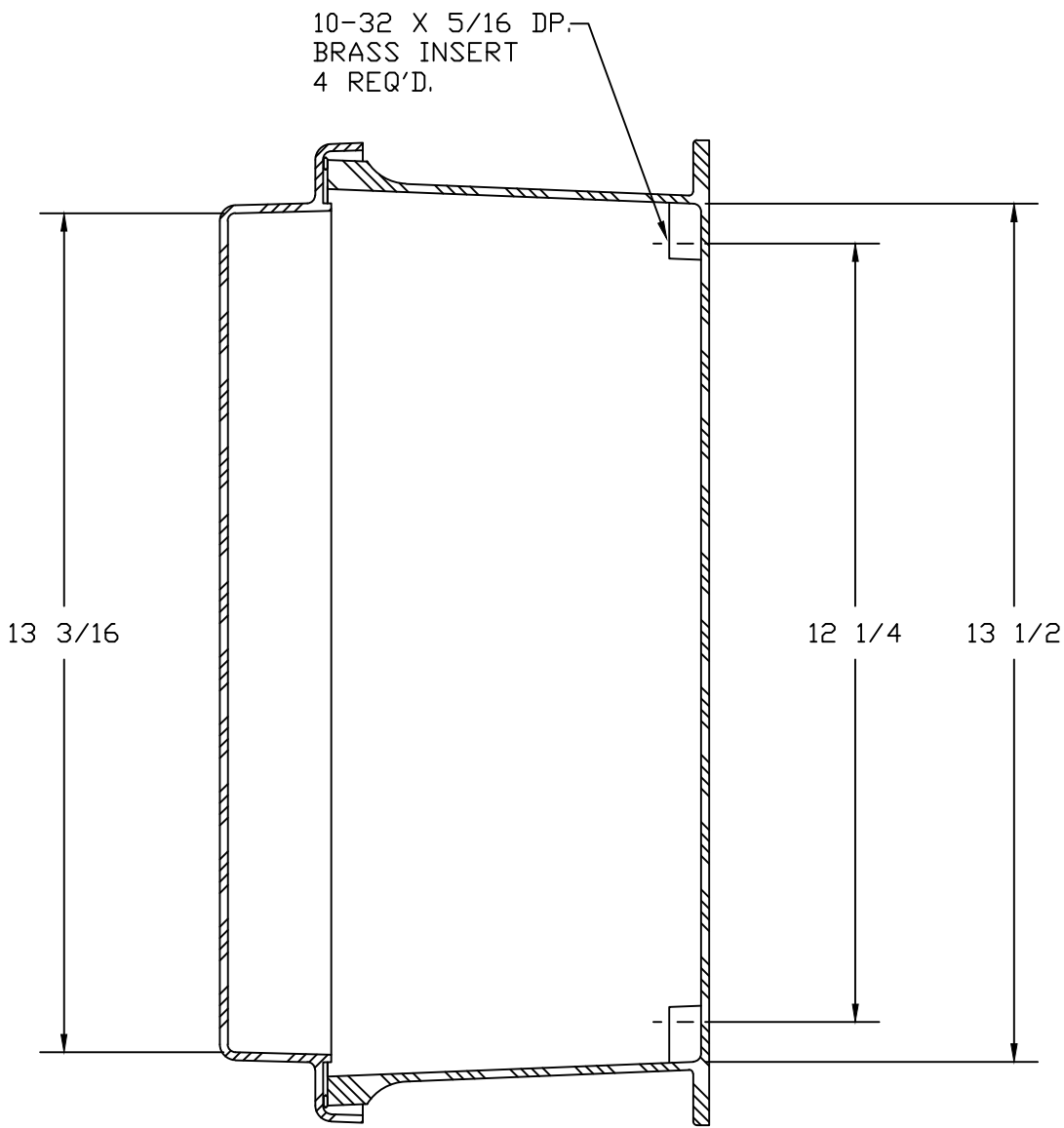
SECTION B-B
