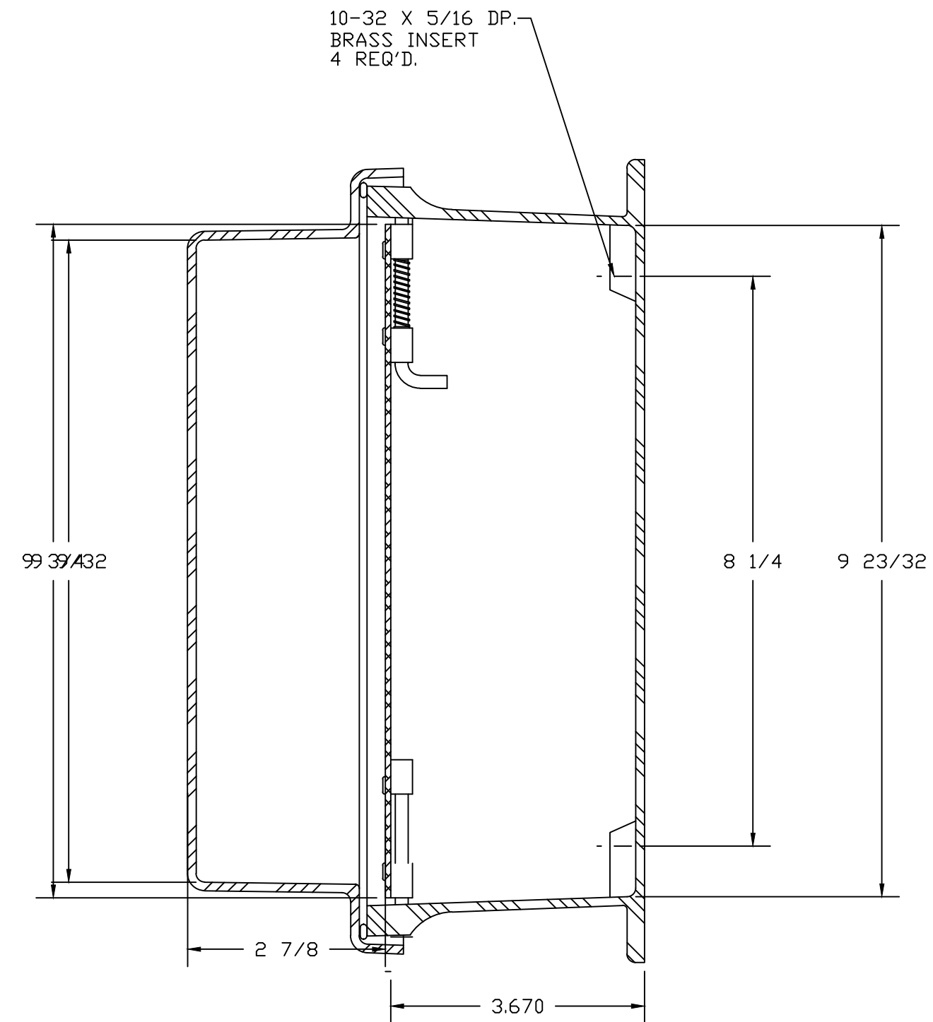
SECTION B-B
