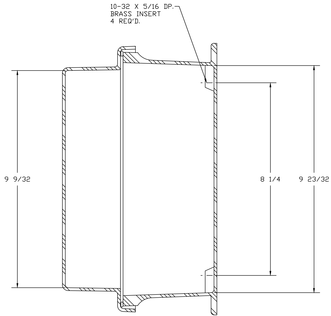
SECTION B-B
