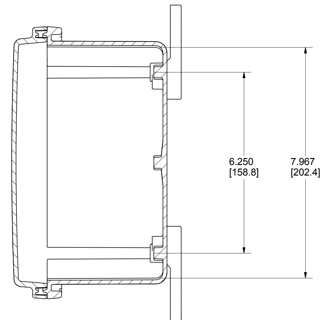
SECTION B-B
