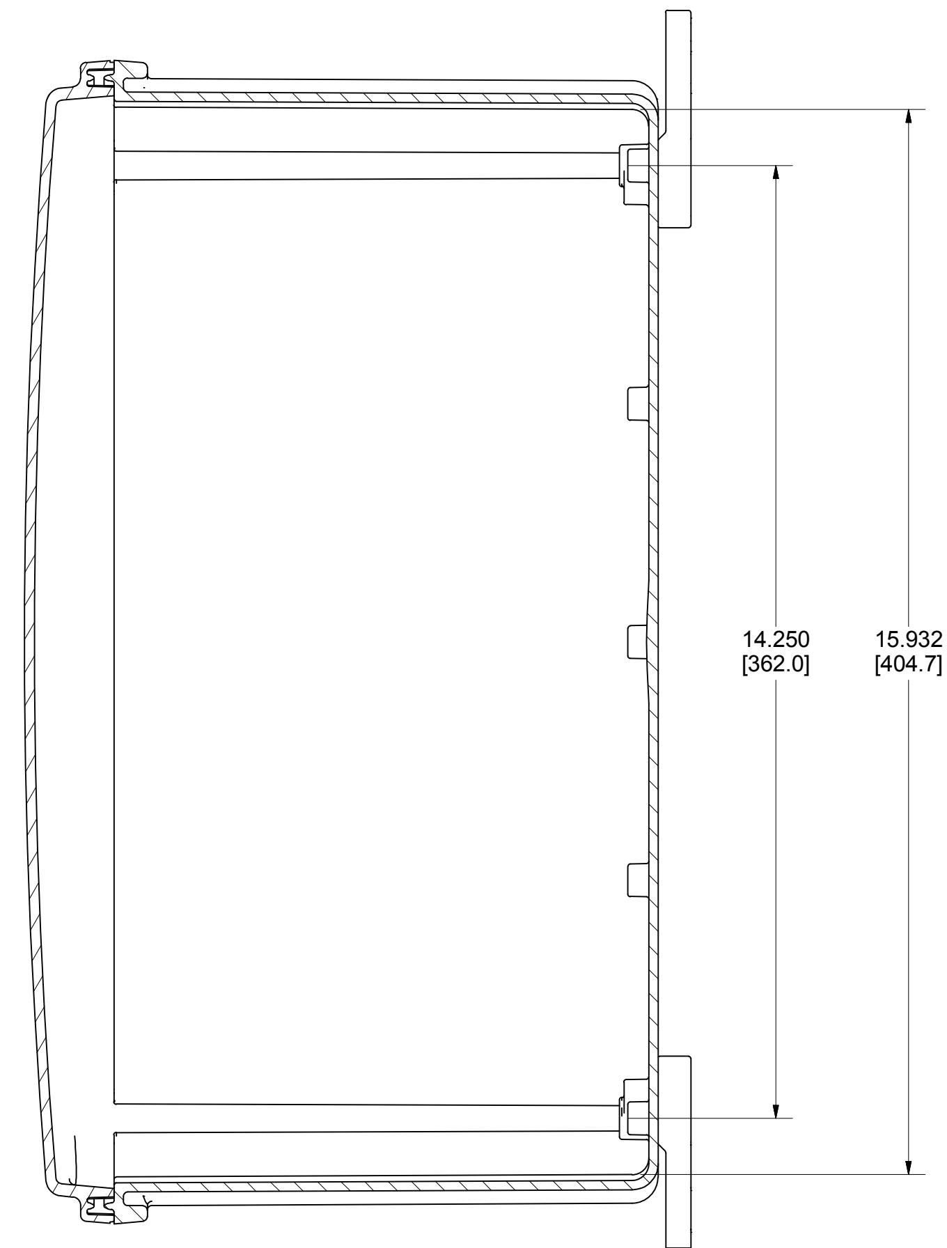
SECTION B-B
