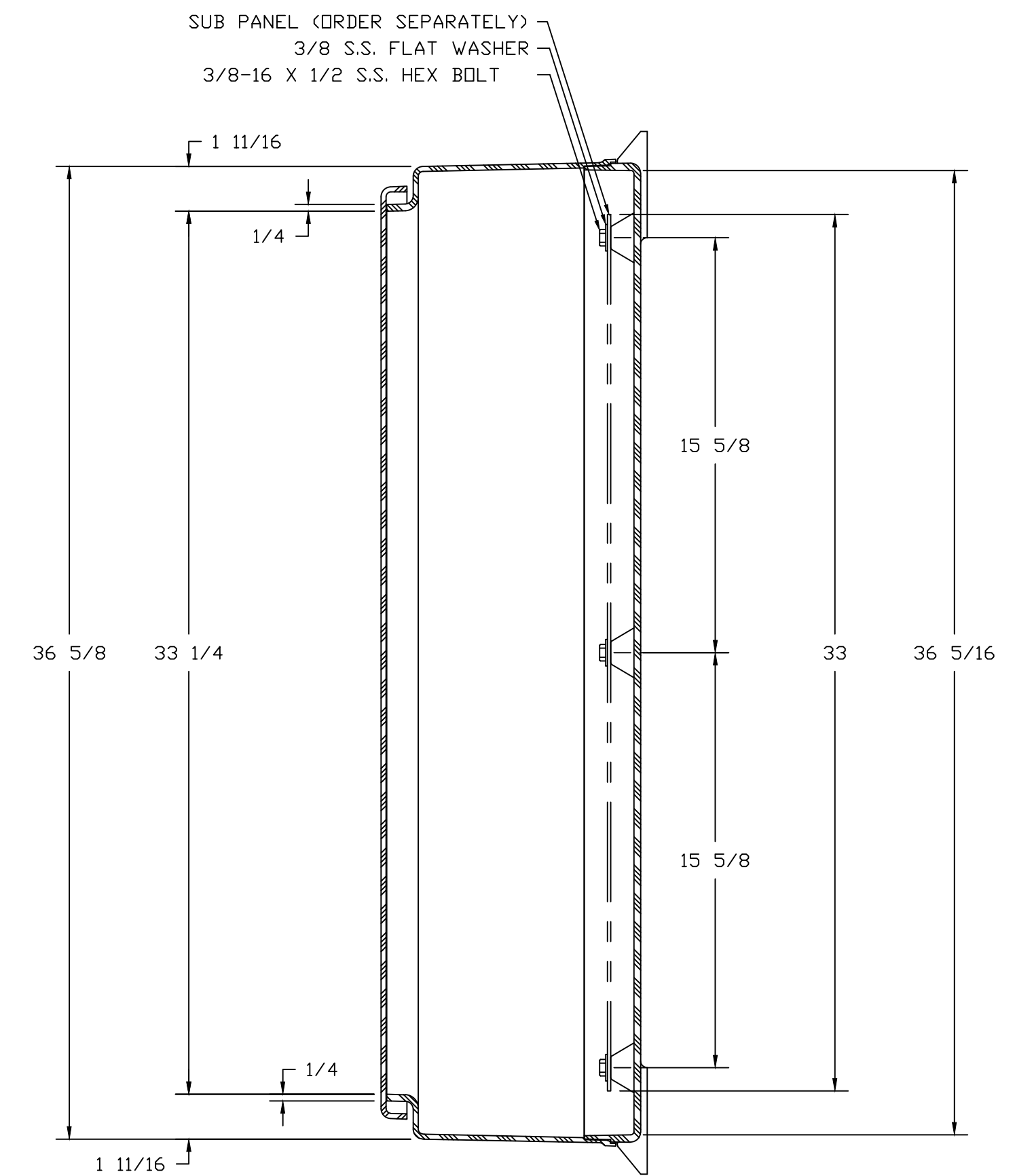
SECTION B-B
