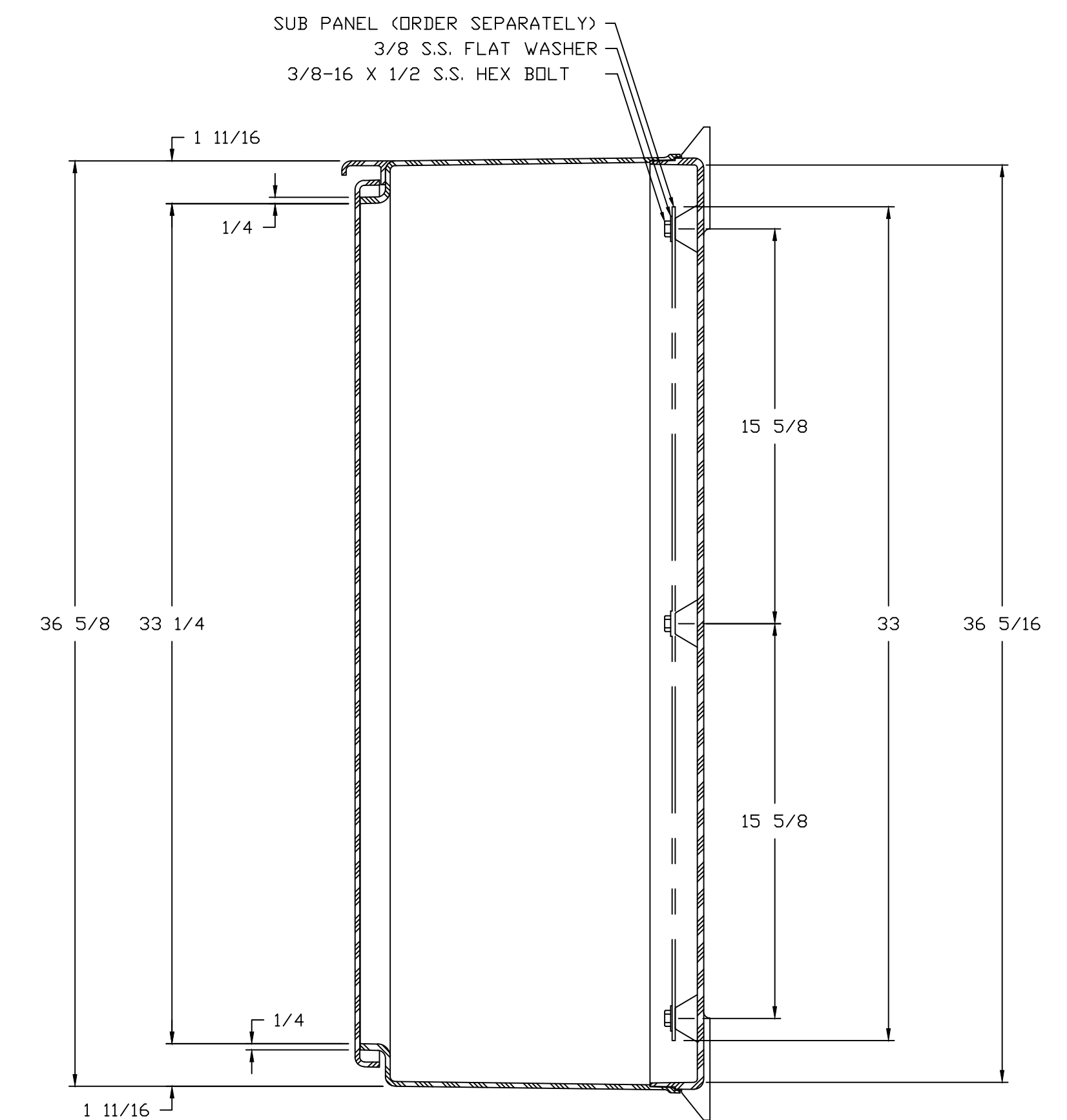
SECTION B-B
