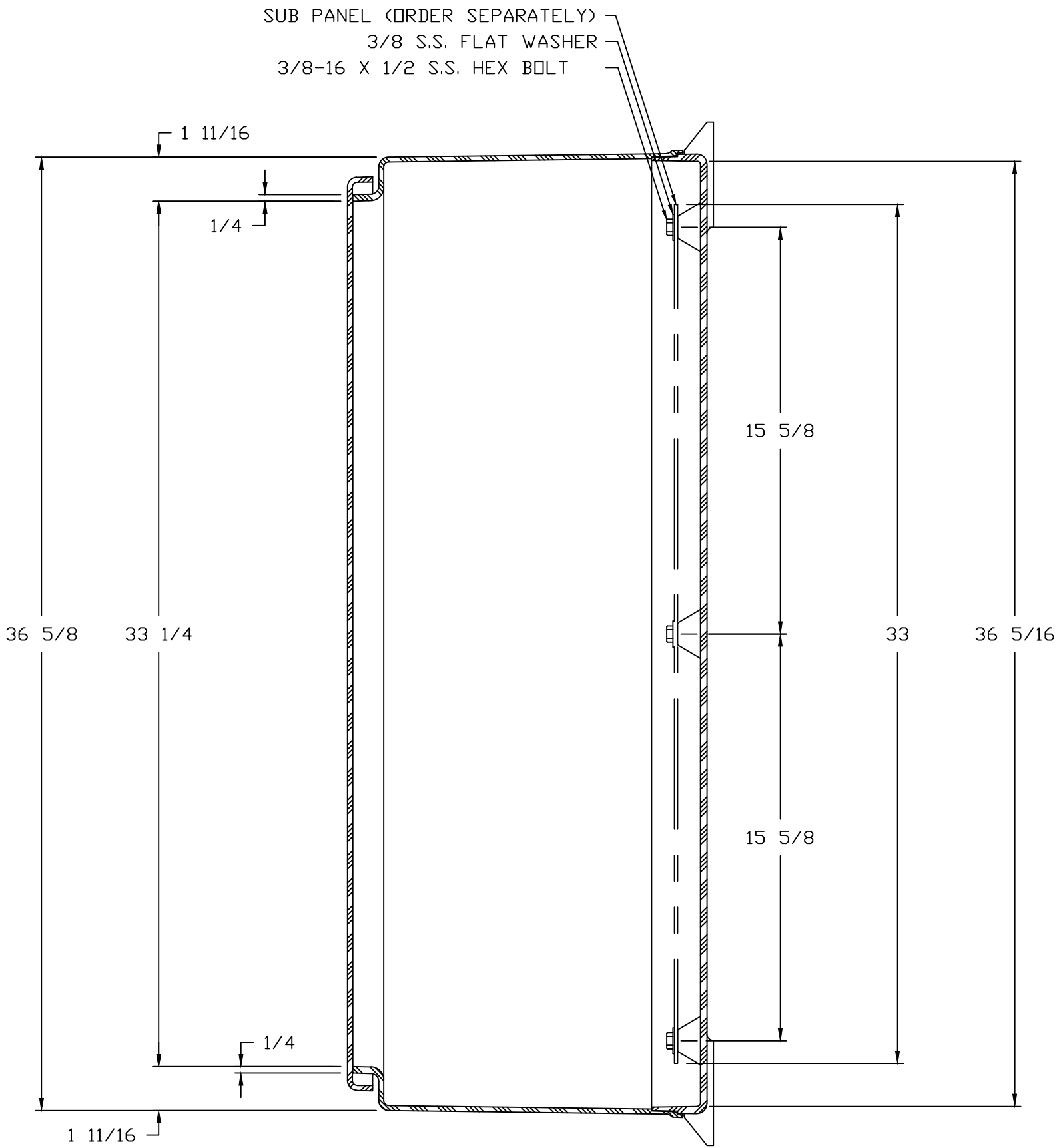
SECTION B-B
