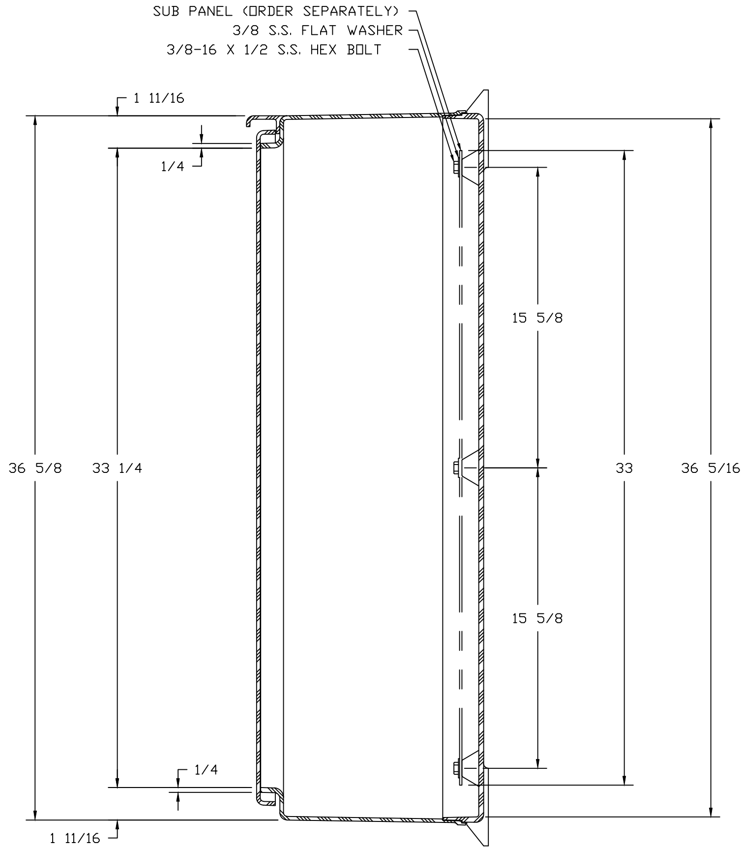
SECTION B-B
