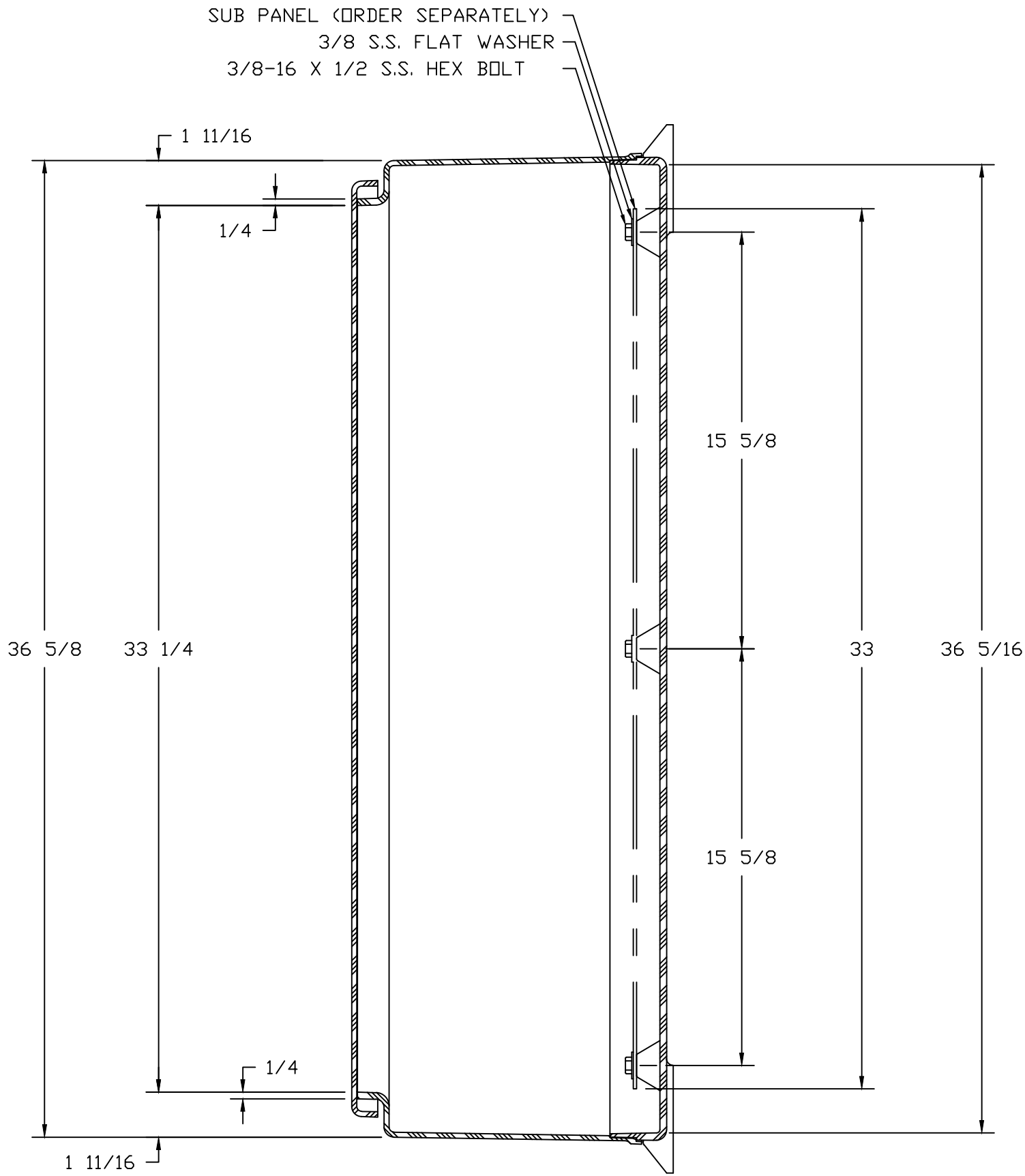
SECTION B-B
