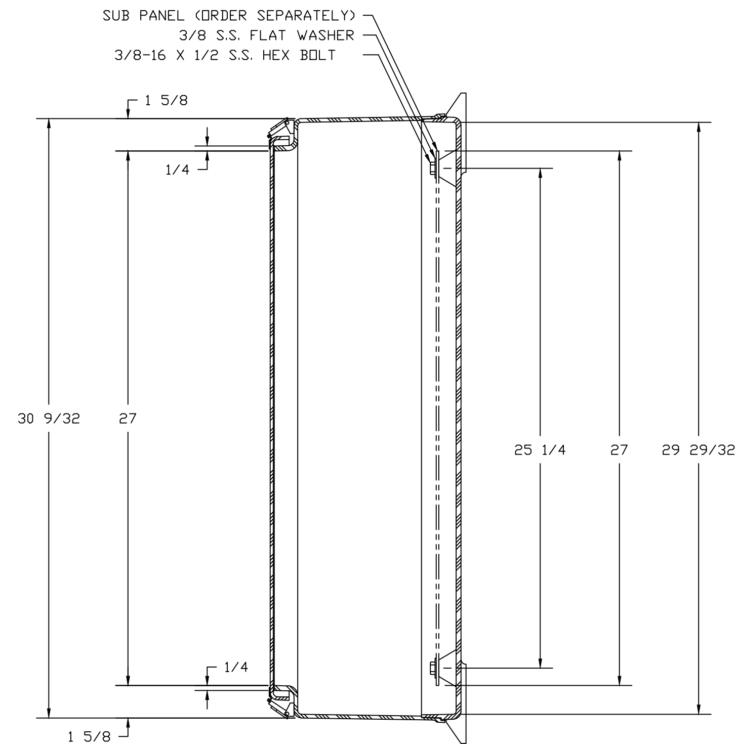
SECTION B-B
