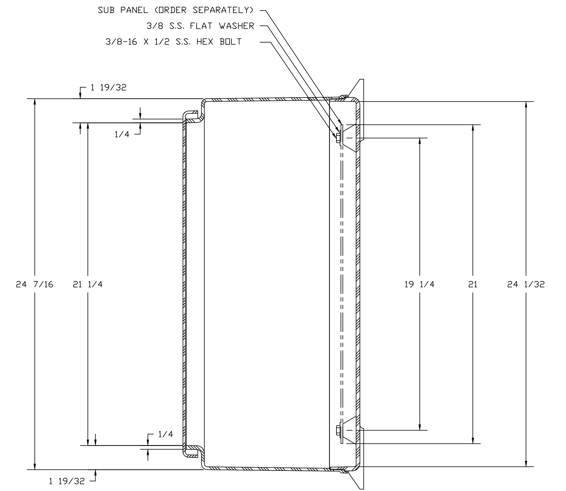
SECTION B-B
