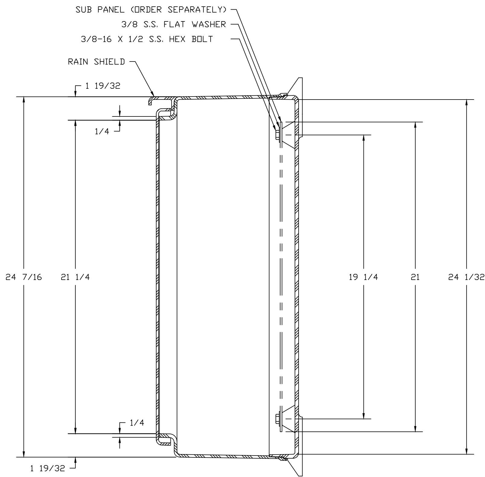
SECTION B-B
