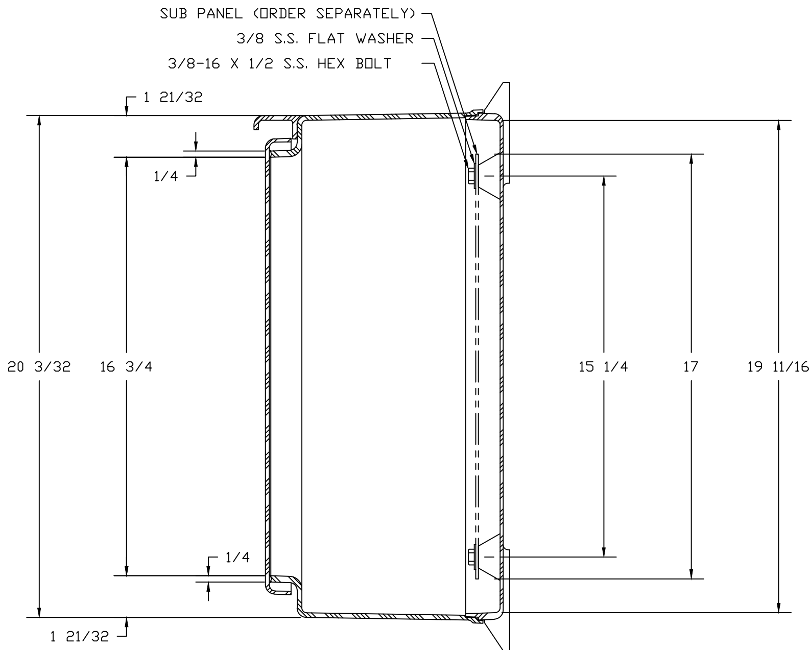
SECTION B-B
