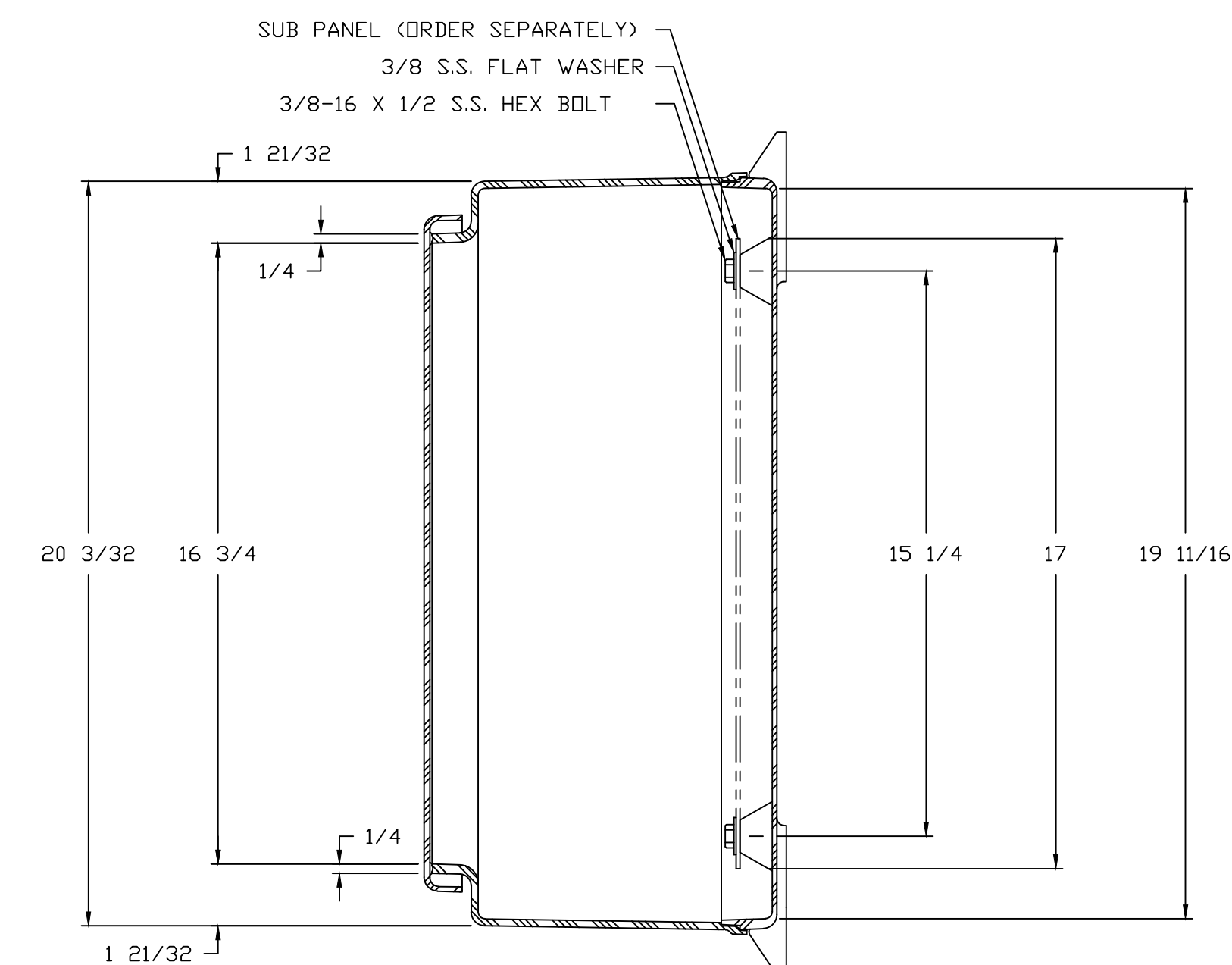
SECTION B-B
