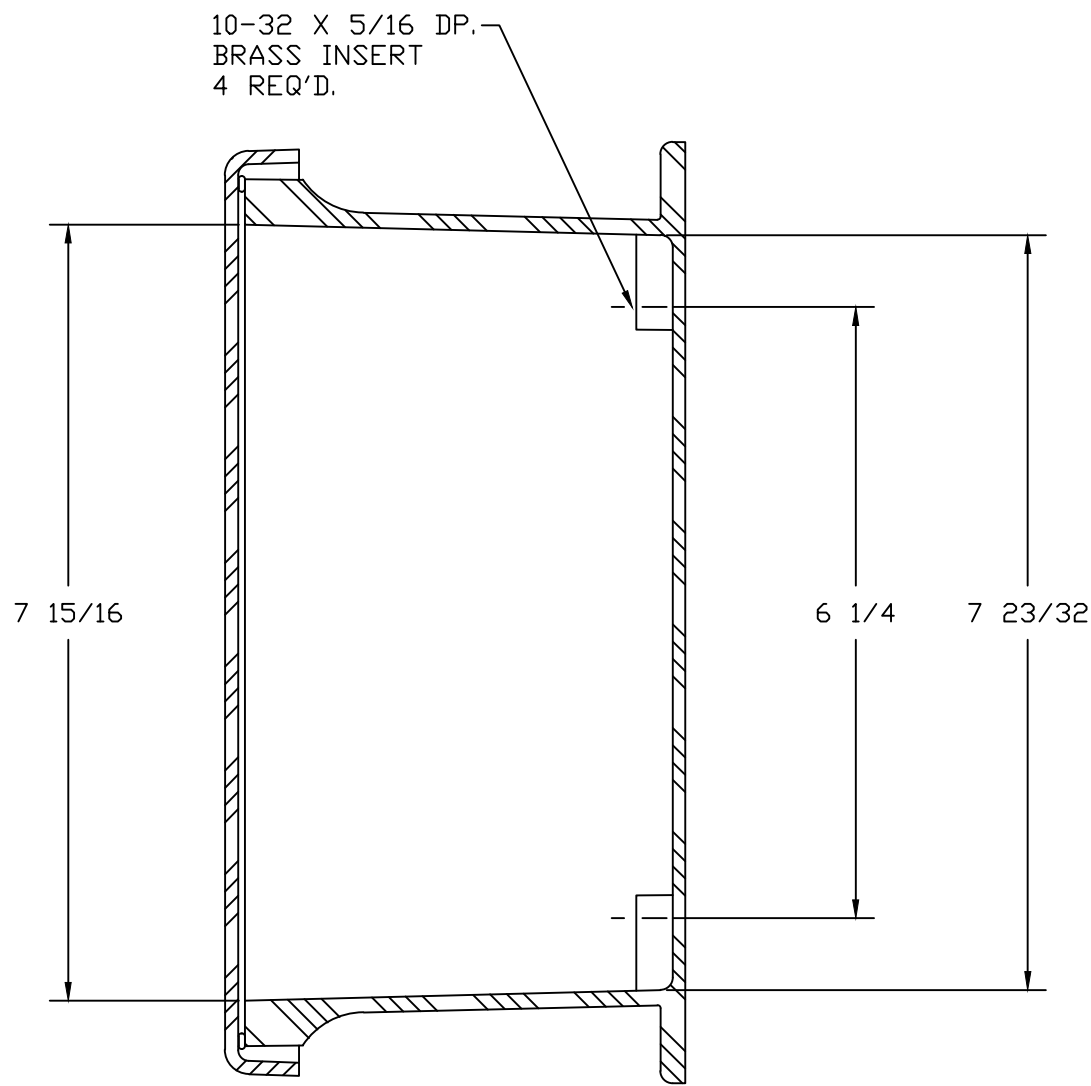
SECTION B-B
