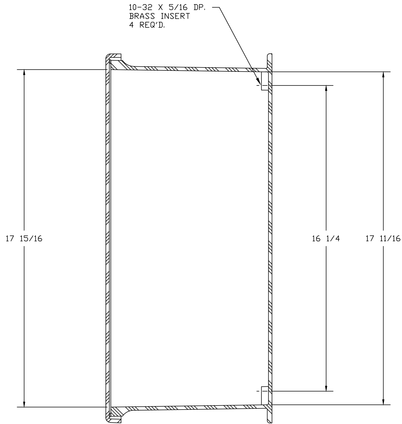
SECTION B-B
