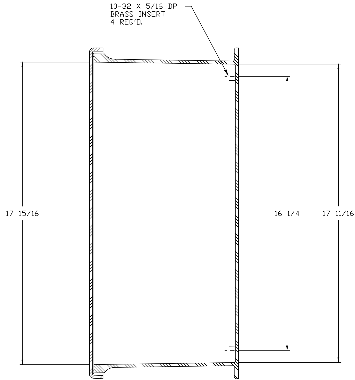
SECTION B-B
