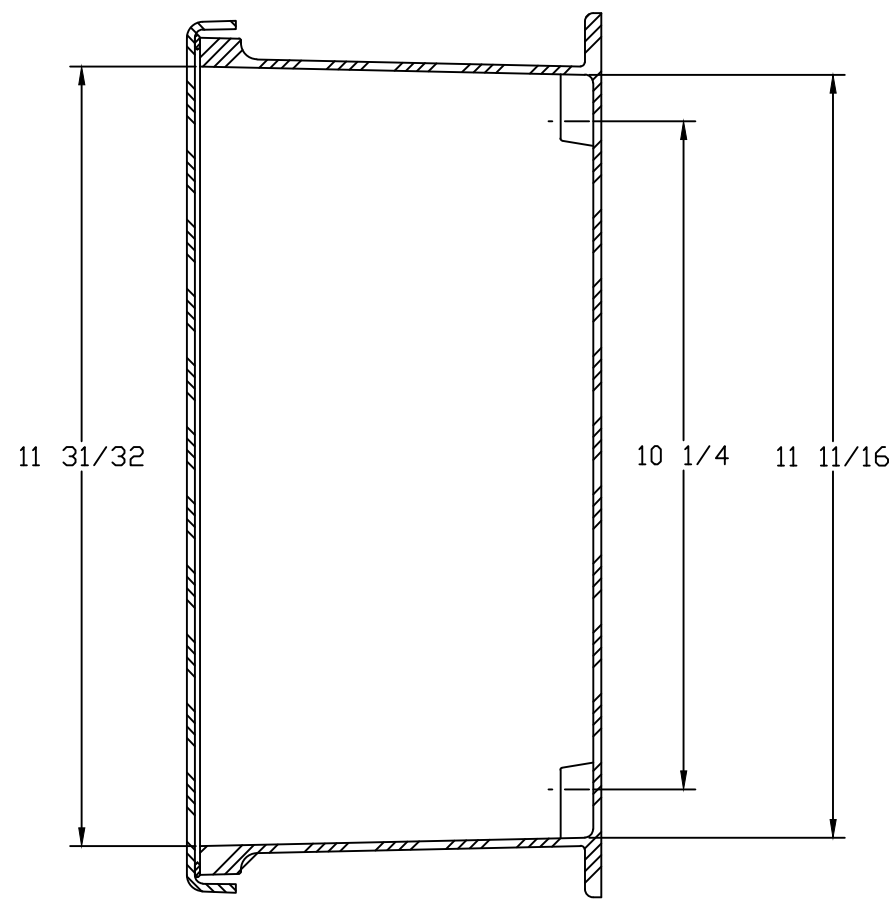
SECTION B-B
