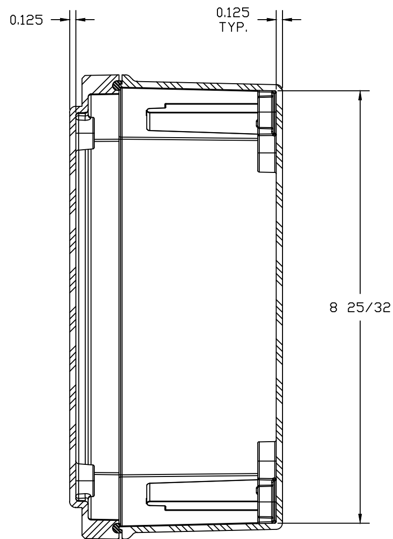
SECTION B-B
