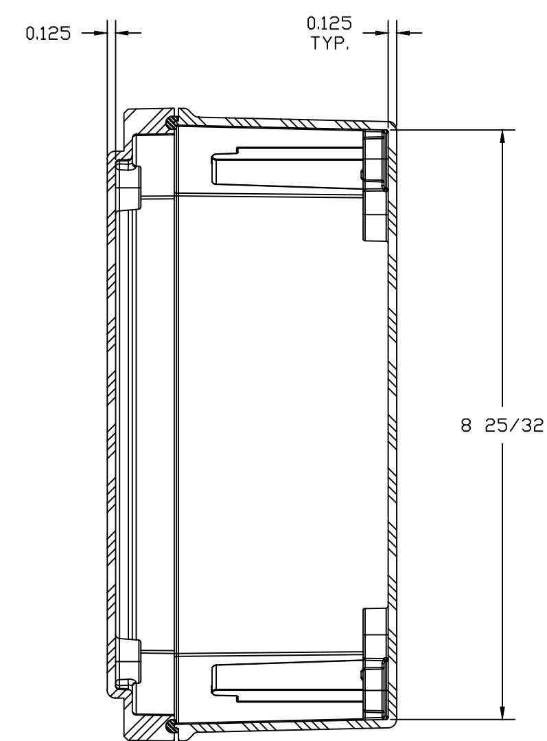
SECTION B-B
