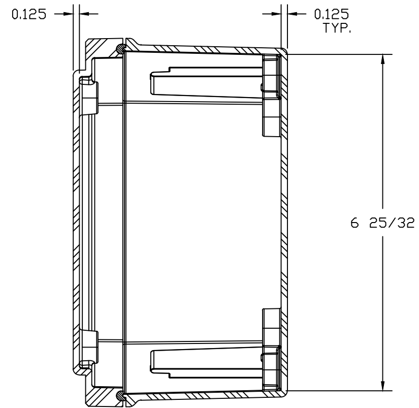
SECTION B-B
