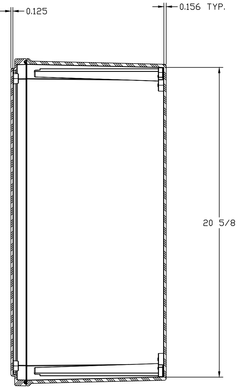
SECTION B-B
