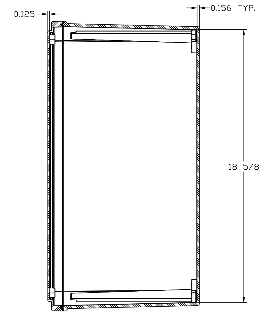
SECTION B-B
