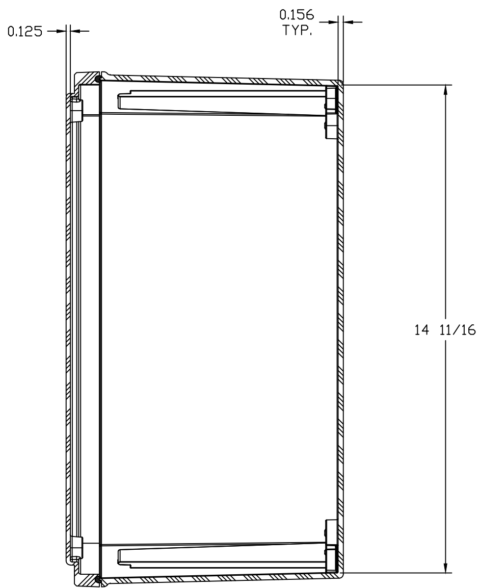
SECTION B-B
