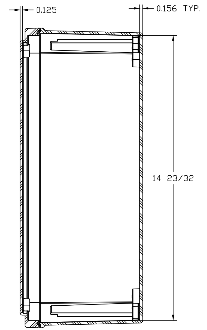
SECTION B-B
