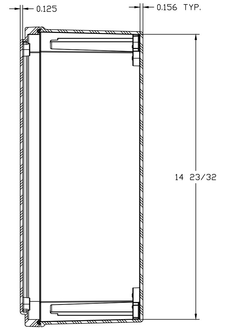
SECTION B-B
