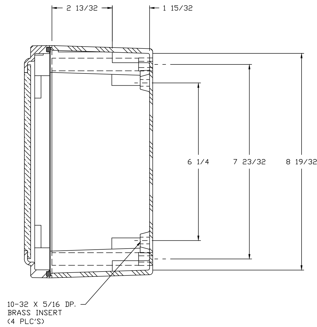
SECTION B-B
