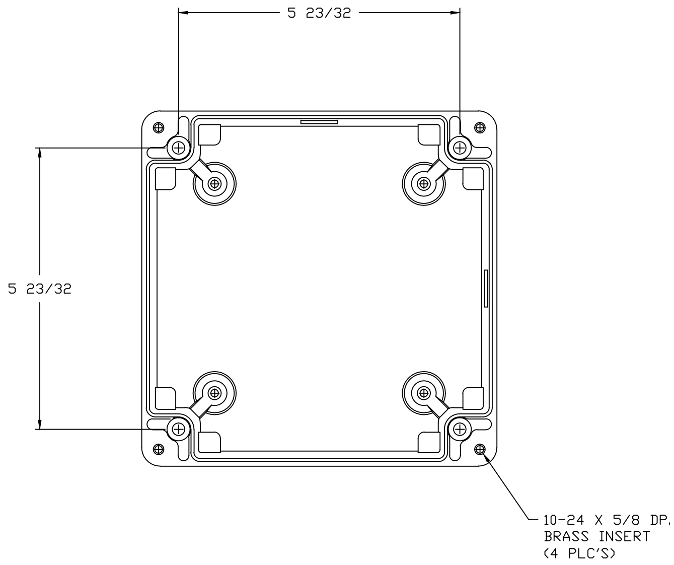
INSIDE VIEW WITHOUT COVER
