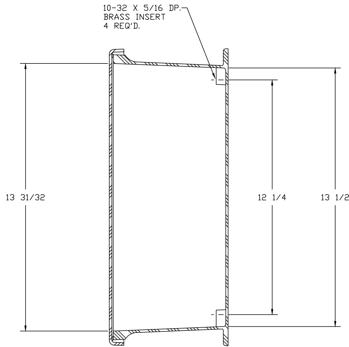
SECTION B-B
