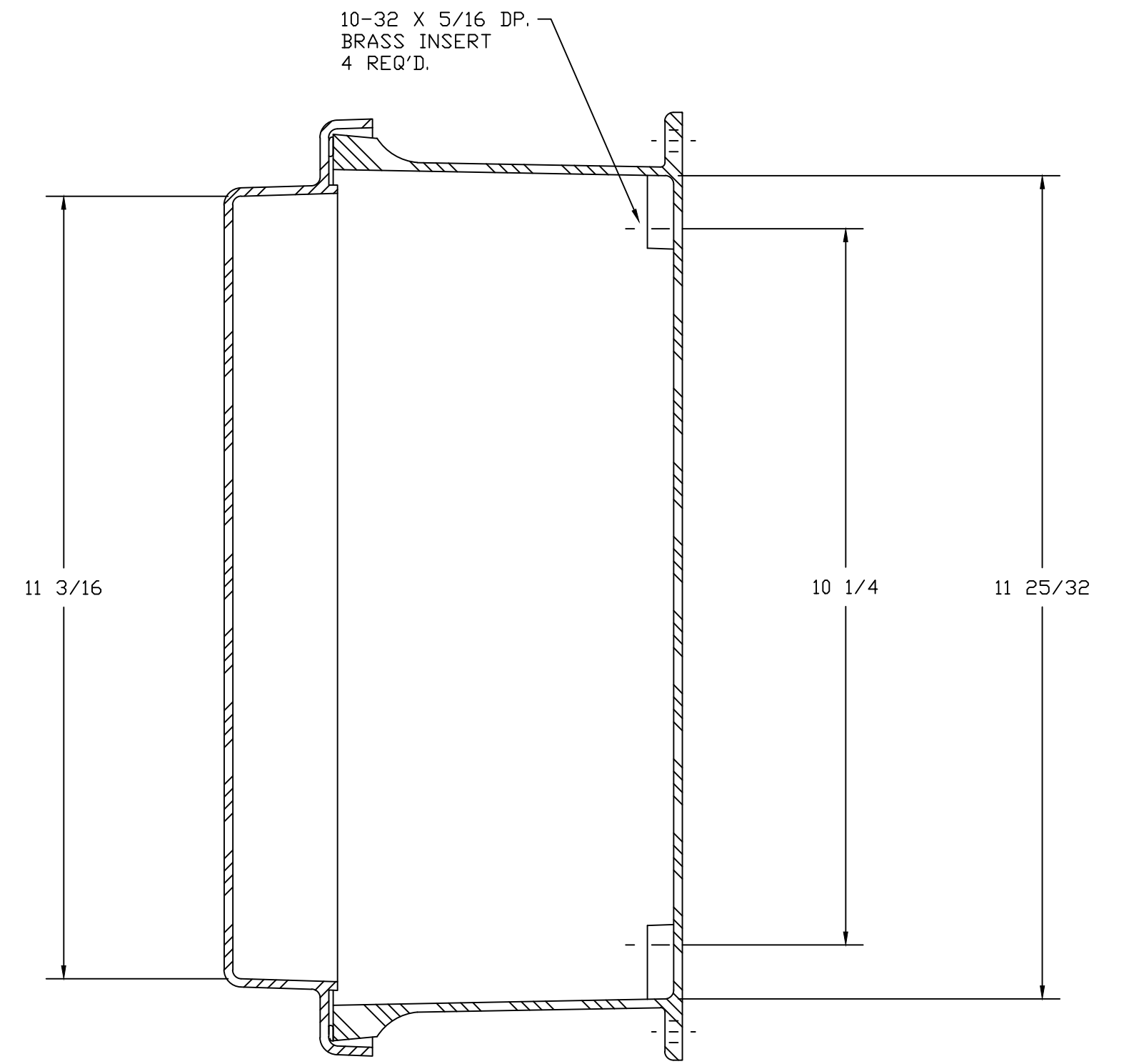
SECTION B-B
