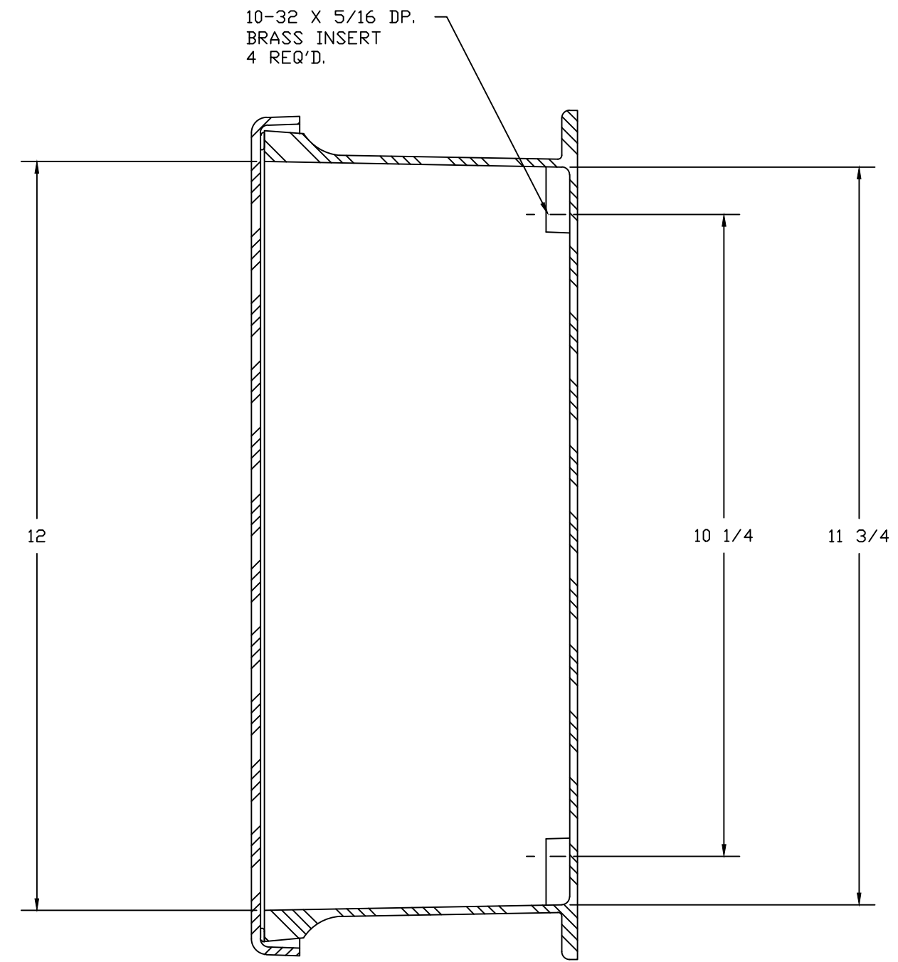
SECTION B-B
