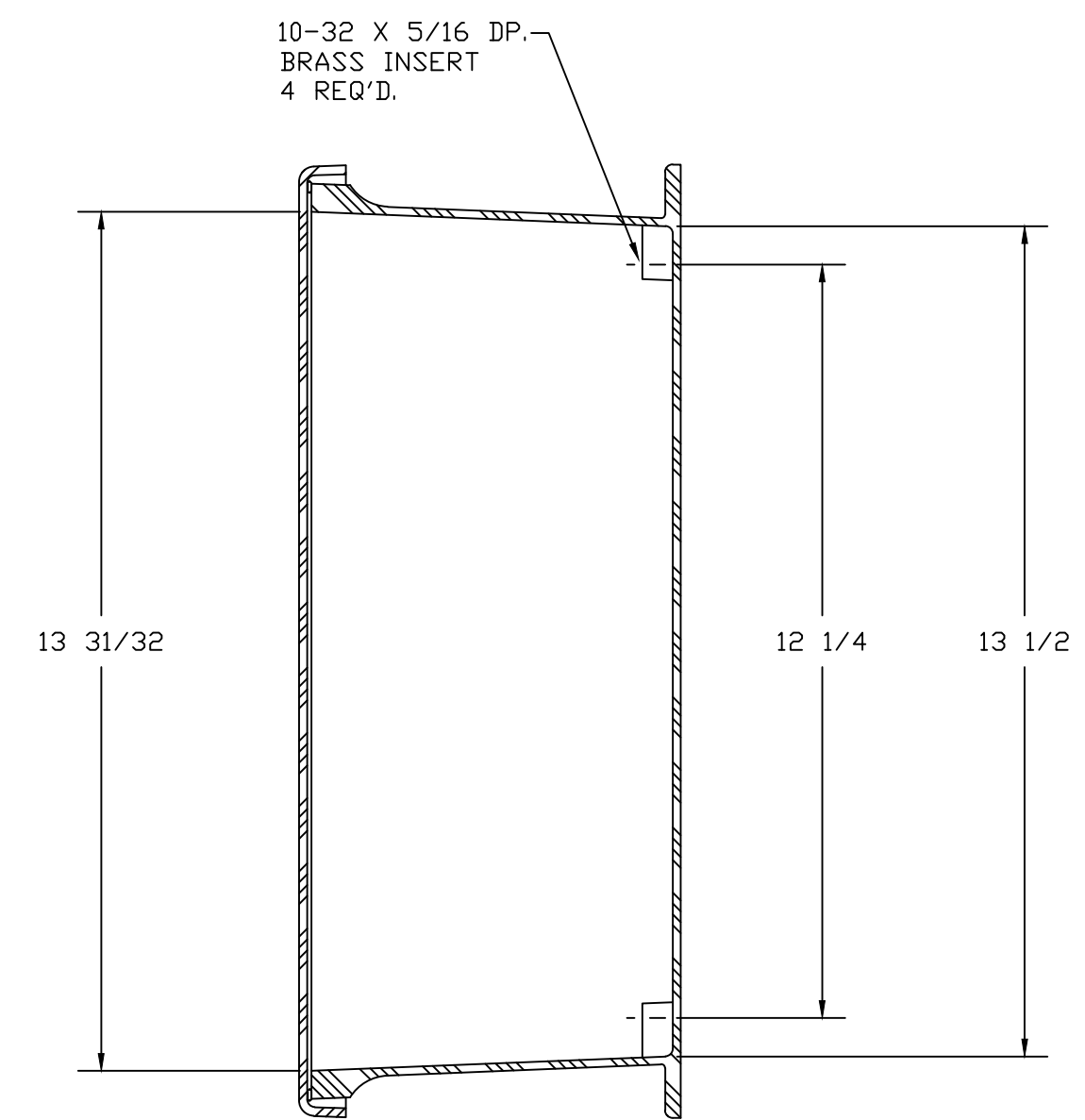
SECTION B-B
