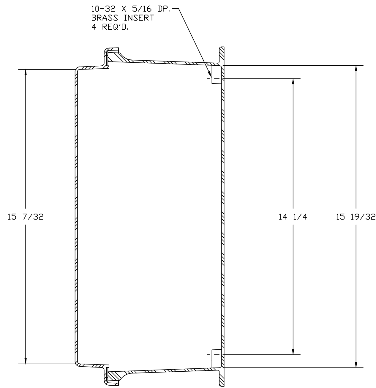
SECTION B-B
