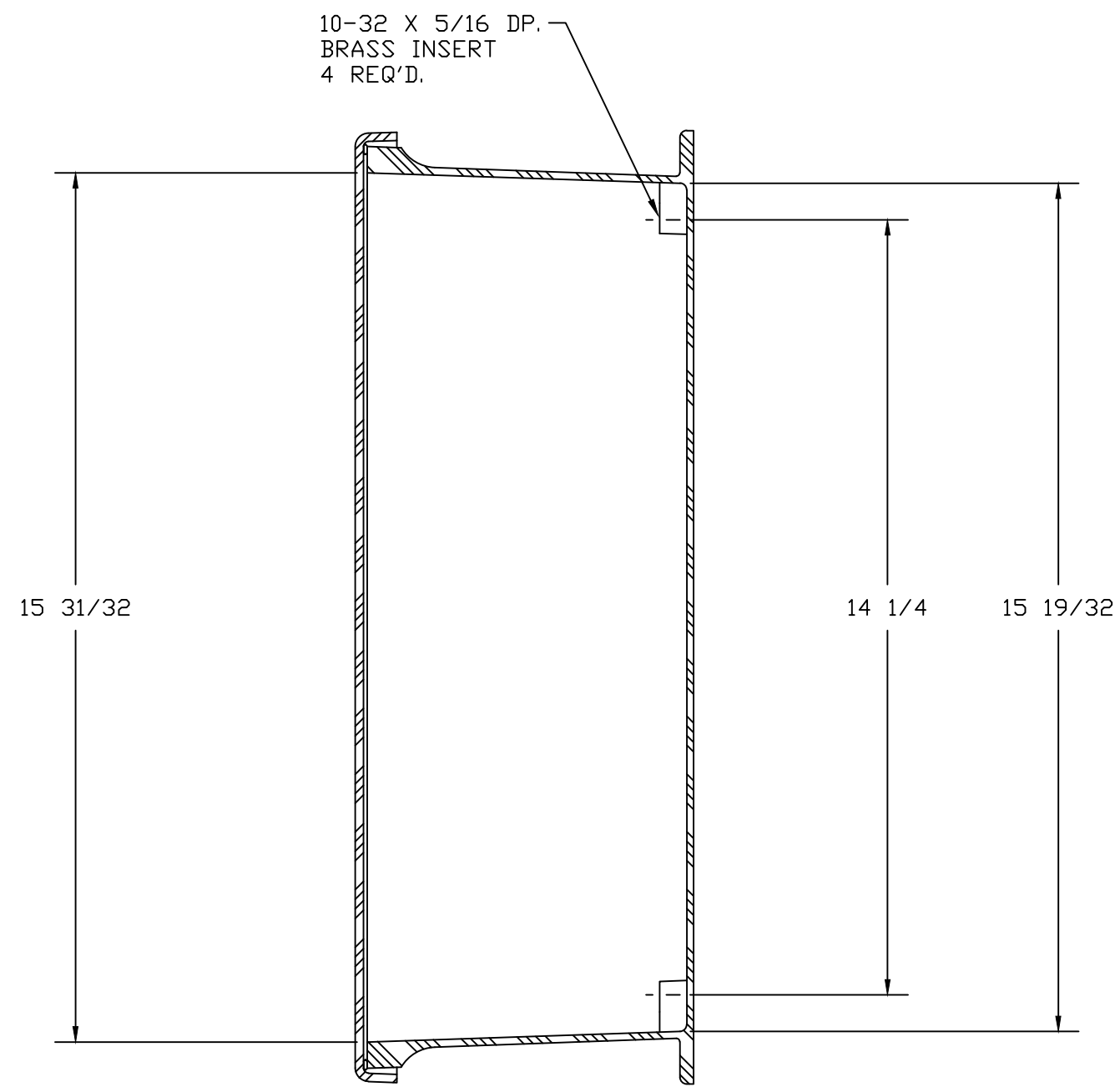
SECTION B-B
