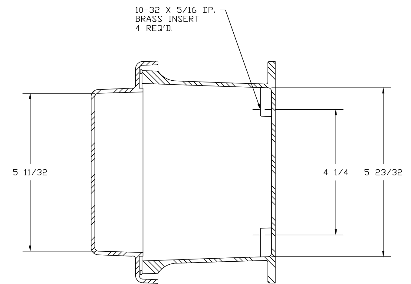
SECTION B-B
