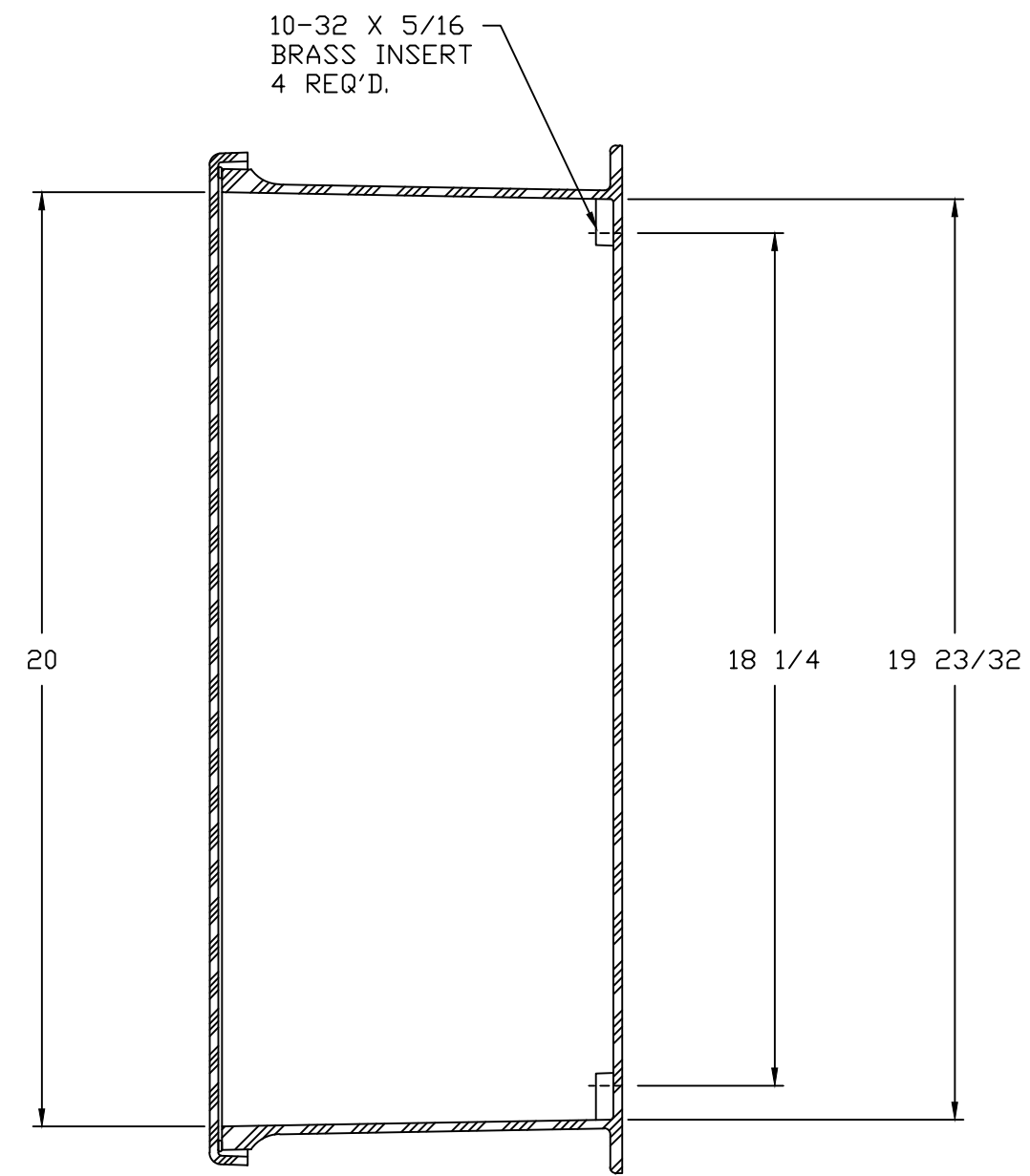
SECTION B-B
