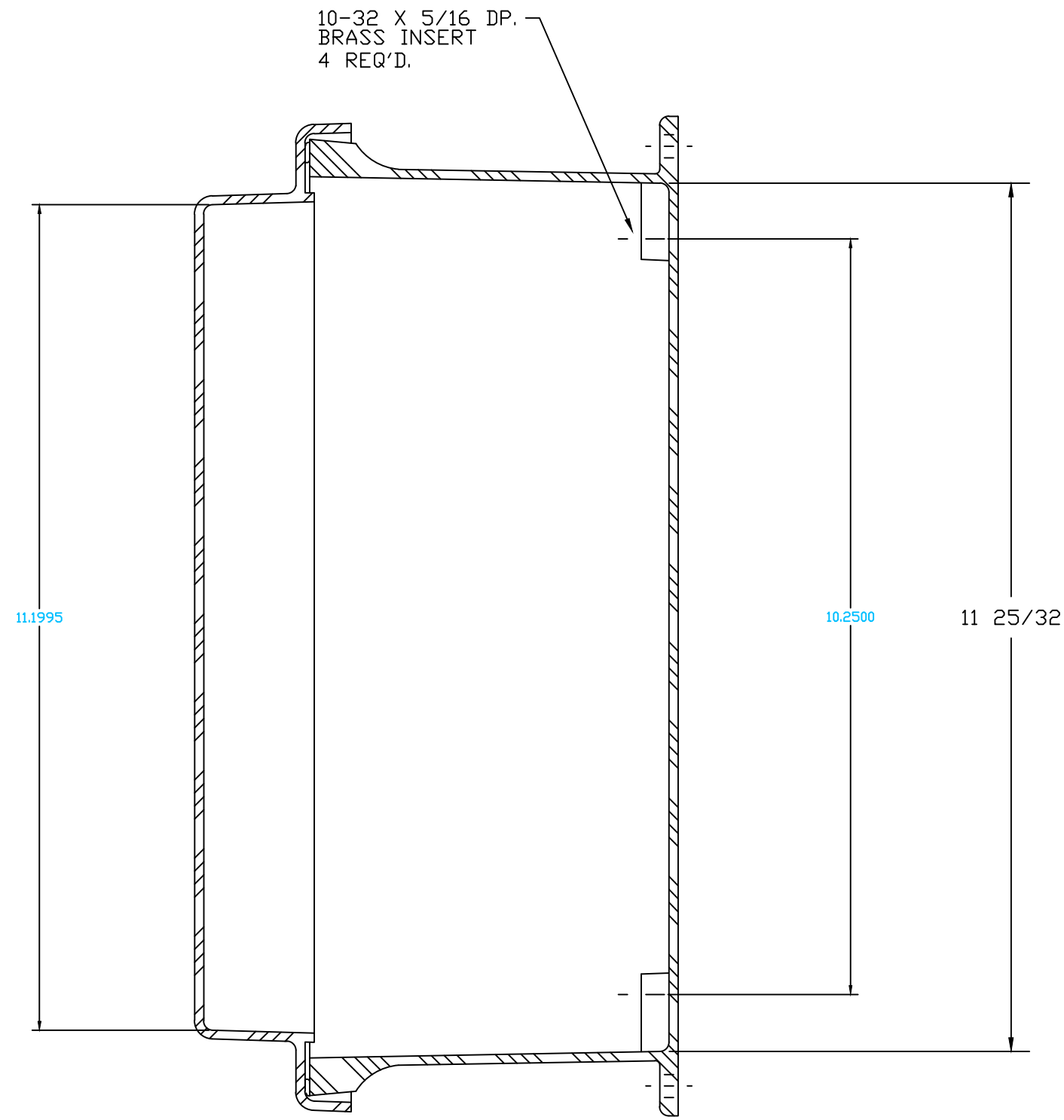
SECTION B-B
